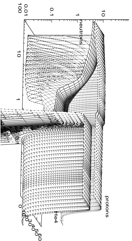
Fig. 1. Number densities of neutrons, protons and 4 \times {}^4\text{He}
