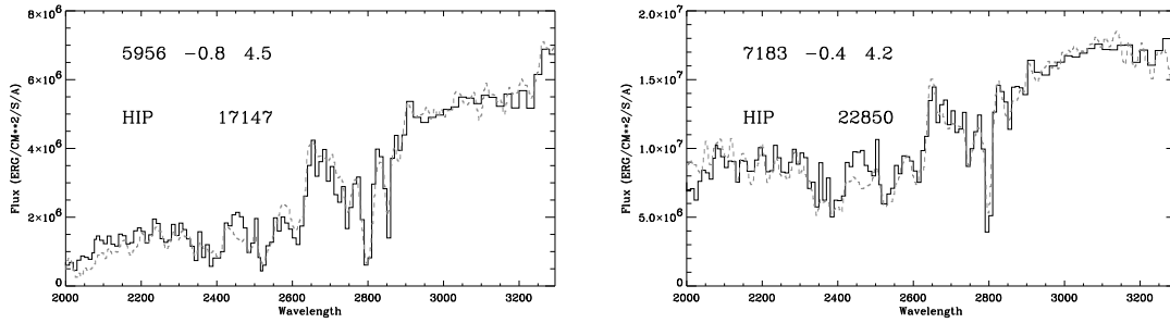
Fig. 1. Two examples of the match between observed (dashed lines) and theoretical (solid lines) absolute fluxes at the stellar surface in the region between 2000 and 3000 Å. Within the panels, T_{\text{eff}} (°K), [\text{Fe}/\text{H}] (dex) and \log g (g in cgs) have been printed, as well as the star's identification in the Hipparcos catalogue.
