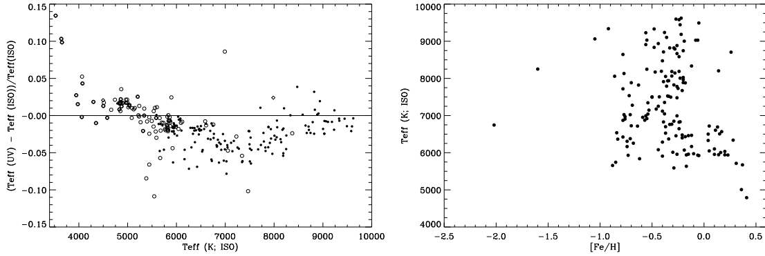
Fig. 2. Left panel: Differences between the effective temperatures derived from the comparison of the star's position in the colour–magnitude diagram with evolutionary isochrones (labeled ISO) and those from fitting the near–ultraviolet continuum (labeled UV). Stars with strong Mg II 2852 Å emission are identified with rhombi, those with a continuum in the region 2000–2400 Å much stronger than predicted by the models with open circles, and the rest with filled circles. Right panel: Position of the normal stars (whose spectra do not show evidence for a chromosphere), on the [\text{Fe}/\text{H}] – T_{\text{eff}} plane. Two stars stand out from the rest, one is the halo star HD 84937 (HIP 48152; [\text{Fe}/\text{H}] \simeq -2.0 ) and the other is HD 192640, a well-known \lambda Bootis star. The two hot stars with [\text{Fe}/\text{H}] \simeq -1.0 are both peculiar too – HD 161868 is a spectroscopic binary and HD 177724 has been assigned a spectral type A0Vpnn by Abt & Morrell (1995).
