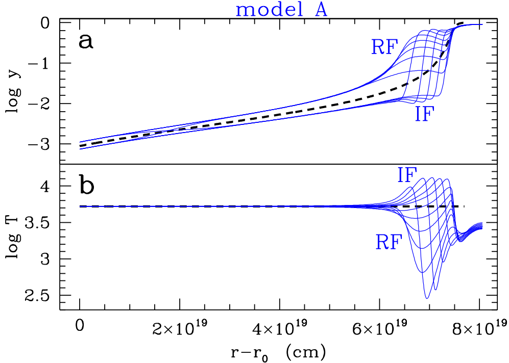
Fig. 2. Internal structure of the nebula as a function of geometrical depth for Model A (cf. § 2.3) assuming a square-wave variability of amplitude A = 0.20 . (a) The neutral fraction y of H. (b) The local temperature T . The long-dashed line represents the initial equilibrium model. The 10 solid lines correspond to the ionization and thermal structure at equally spaced time intervals during the last full cycle shown in Fig. 1a.
