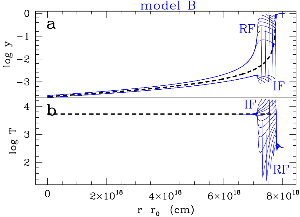
Fig. 3. Internal structure of the nebula as a function of geometrical depth for Model B (cf. § 2.6) assuming a square-wave variability of amplitude A = 0.10 . (a) The neutral fraction y of H. (b) The local temperature T . The long-dashed line represents the initial equilibrium model. The 10 solid lines correspond to the ionization and thermal structure at equally spaced time intervals during the last full cycle.
