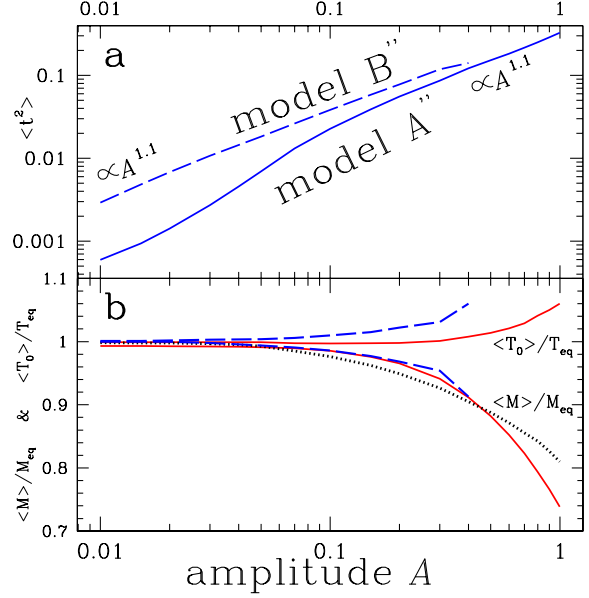
Fig. 5. (a) Behavior of \langle t^2 \rangle as a function of the amplitude of the sine-wave variations of Q_H . (b) Behavior of \langle \bar{T}_0 \rangle / T_{eq} (curves \geq 1 ) and \langle M \rangle / M_{eq} (curves \leq 1 ) as a function of the amplitude of the sine-wave variations. Model A'' and B'' are represented using solid and dashed lines, respectively. The dotted line represents the equation (1 + 0.7863 \langle t^2 \rangle)^{-1.177} \langle \bar{T}_0 \rangle / T_{eq} (see § 2.8) using values from Model A''. Model B'' was not computed beyond A = 0.4 .
