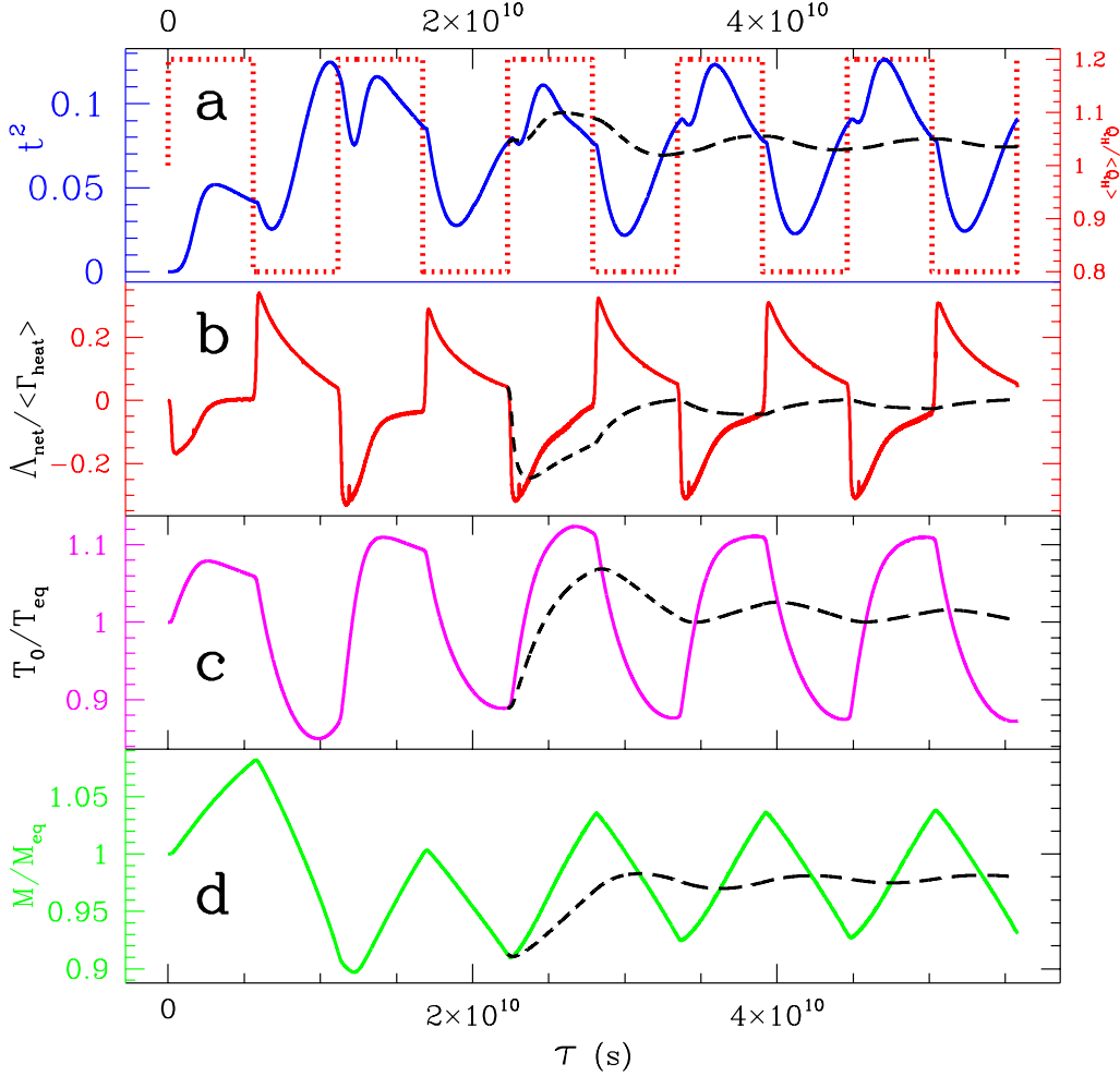
Fig. 1. Behavior of nebular volume-weighted quantities (solid lines) as a function of time \tau for Model A. (a) t^2 . (b) Net cooling relative to the mean heating energy radiated by the source \Lambda_{\text{net}}/\langle\Gamma_{\text{heat}}\rangle [with \langle\Gamma_{\text{heat}}\rangle = h(\bar{\nu} - \nu_0)\langle Q_{\text{H}}\rangle ]. (c) The mean electron temperature \bar{T}_0/T_{\text{eq}} . (d) The mass of ionized gas M/M_{\text{eq}} . In each panel, the long-dashed line across the last three cycles represents the running mean of the plotted quantity. The asymptotic values referred to in the text (e.g. \langle\bar{T}_0\rangle , \langle t^2 \rangle ) correspond to the rightmost value along the long-dashed line. The square-wave dotted-line in a is the normalized photon luminosity of the ionizing source as a function of time, Q_{\text{H}}(\tau)/\langle Q_{\text{H}}\rangle (to be read on the upper right y -axis). The variability is characterized by an amplitude A = 0.2 , a period \Pi = \tau_{\text{rec}} and a duty cycle \Delta = 0.5 .
