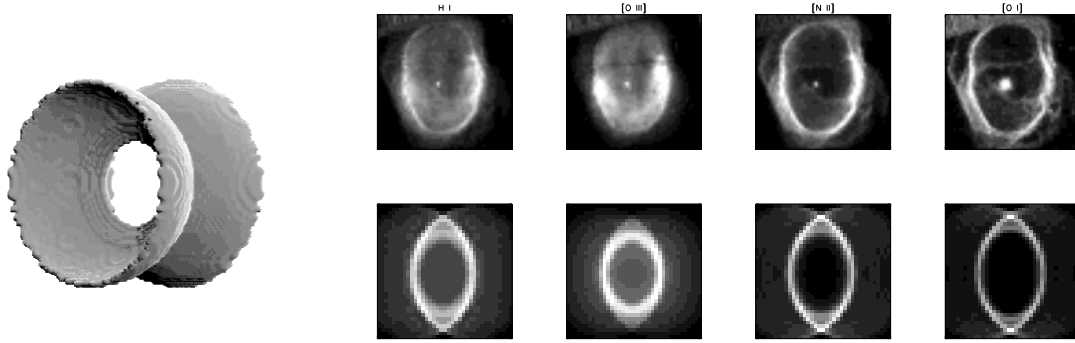
Fig. 1. (Left) The Diabolo shape showing high density region with n = 1300 \text{ cm}^{-3} . The background density is 300 \text{ cm}^{-3} . (Right) HST observations (top) and corresponding line images of the Diabolo model (bottom).
