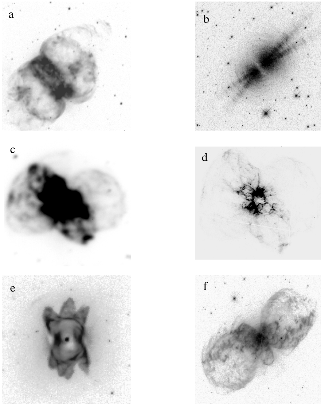
Fig. 1. Bipolarity and poly-polarity in PNe. The presence of equatorial density enhancements (EDE) is a key ingredient in the formation of bipolar nebulae. The mechanisms that form EDE are still unknown. Bipolarity develops from the early stages of PN formation (see text). (a) NGC 650 a typical bipolar nebula with a conspicuous EDE. (b) The proto-PN CRL 2688 already showing clear signs of bipolarity and concentric shells. (c) NGC 2440 a poly-polar nebula with more than one pair of opposing lobes. (d) NGC 2440 ( HST ), the inner regions and secondary lobes revealed. (e) He 2–339 ( HST ), a young poly-polar nebula. (f) Hb 5 ( HST ), a bipolar nebula with a point-symmetric structure along the inner borders of its opposing lobes. Credits for the images: (a) López (and see Bryce et al. 1994) (b) Sahai & Trauger and WFPC2 Science Team. (c) López (d) Westphal, and see López et al. (1998) (e) Sahai & Trauger (f) Balick, Icke, & Mellema.
