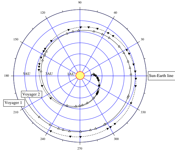
Fig. 2. Voyager 1 and 2 trajectories as seen from a corotating reference frame where the line Sun-Earth is fixed. The trajectories cover a heliocentric range from 1 to 5.4 AU.
