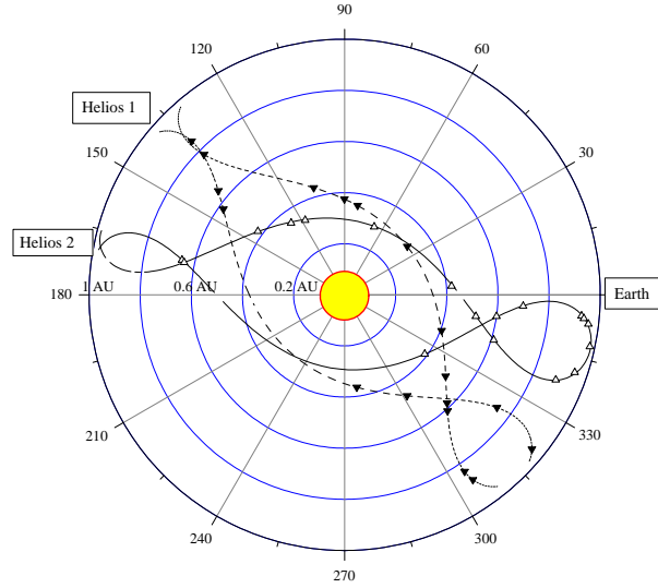
Fig. 1. Helios 1 and 2 trajectories from August 1977 to August 1978 as seen from a corotating reference frame where the line Sun-Earth is fixed. The triangles denote the location where the spacecraft detected the shocks.
